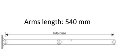
Steel arms
